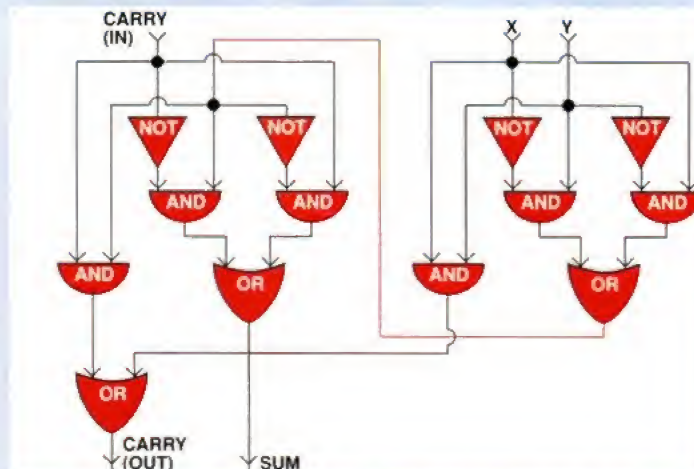
The FULL ADDER is a combination of two or more half adders and an OR gate and can happily handle a sum that involves carrying a leftover digit.
